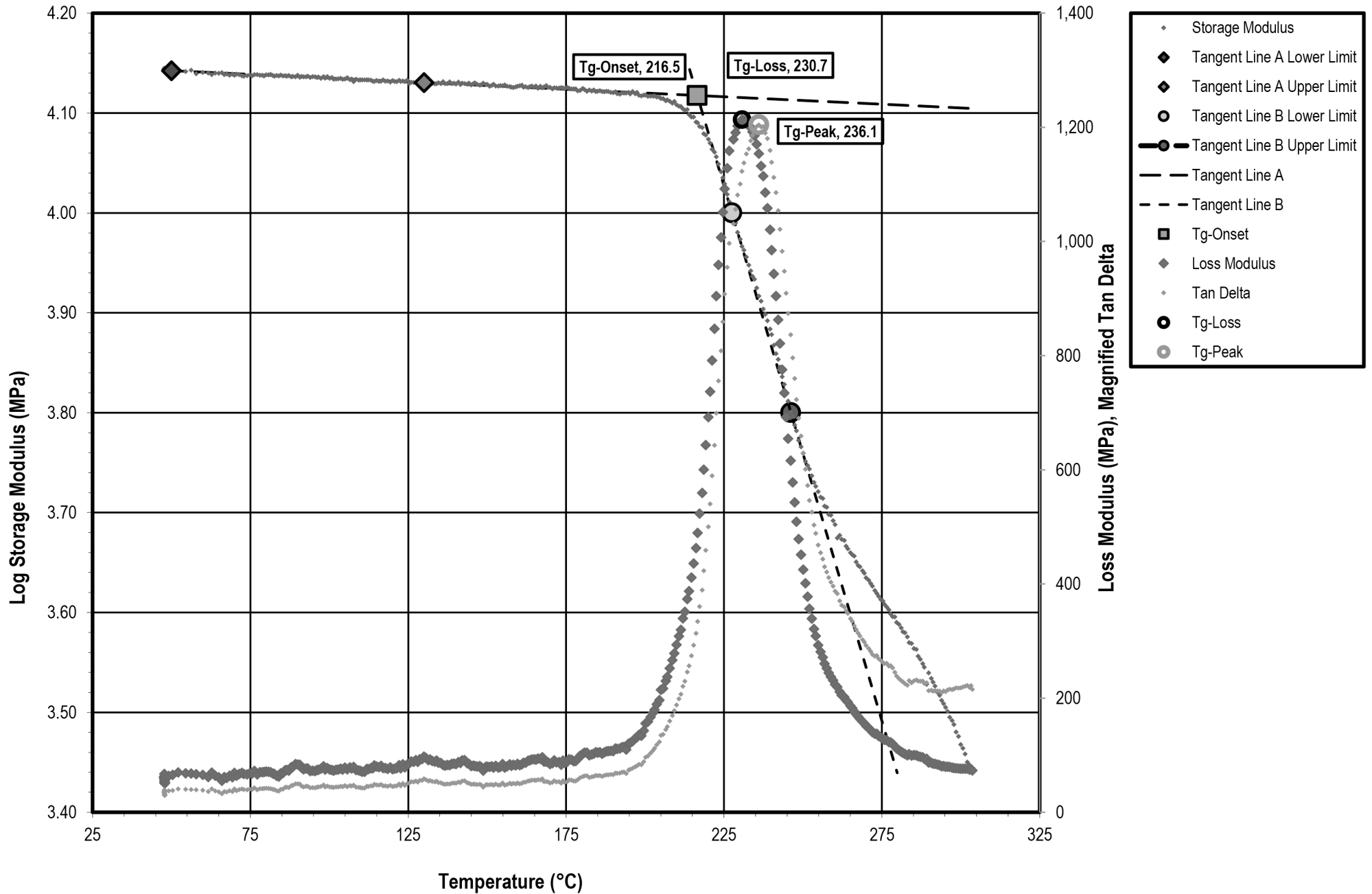
Storage Modulus, Loss Modulus and Tangent Delta vs. Temperature
